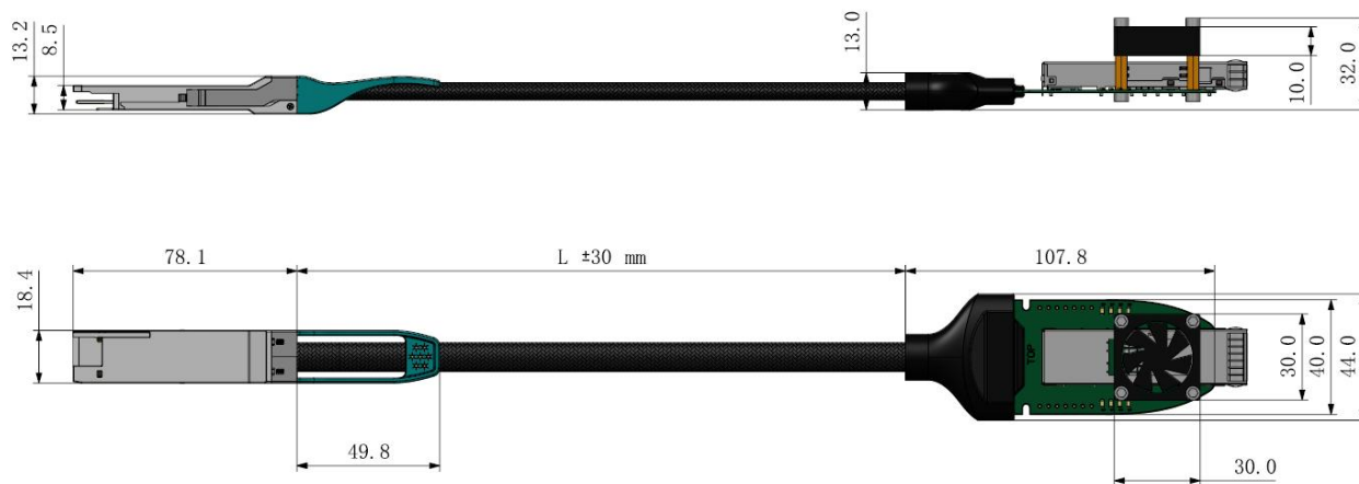
Figure 5. Mechanical Specifications
