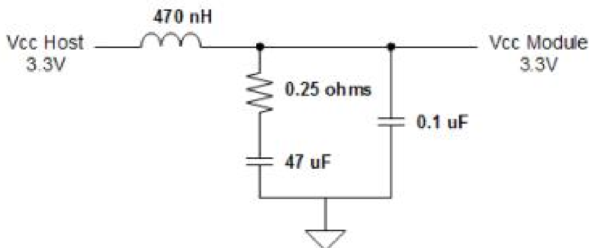
Figure7. Host Board Power Supply Filtering
