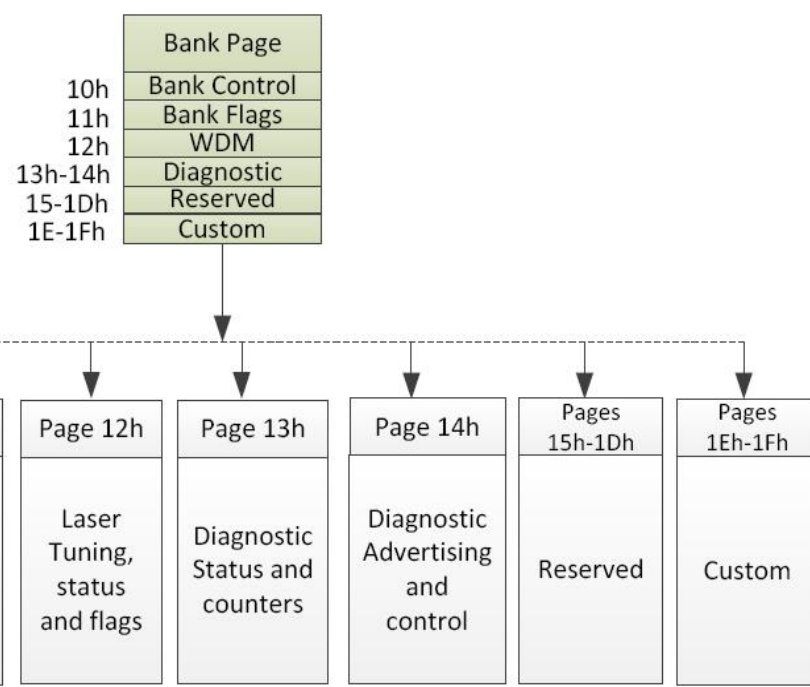
Figure8. OSFP Memory Map
