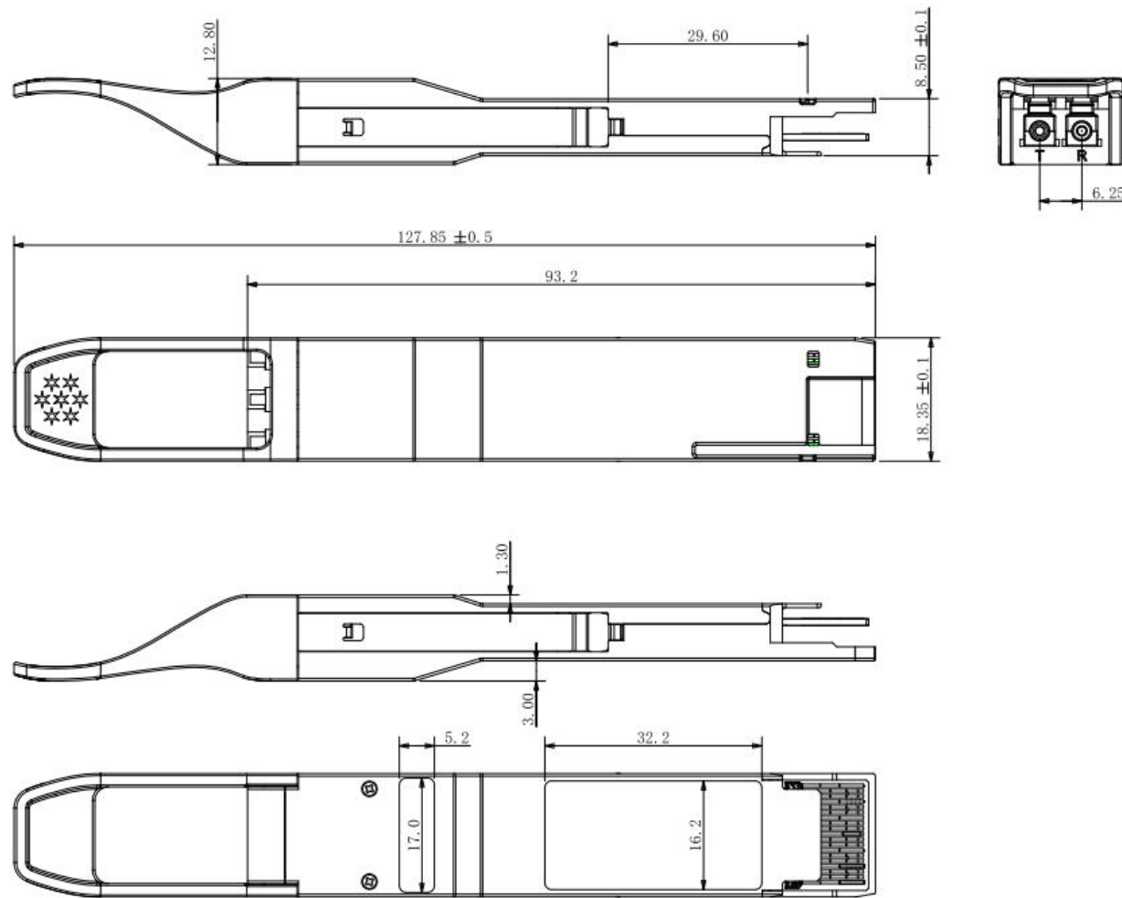
Figure5. Mechanical Specifications
