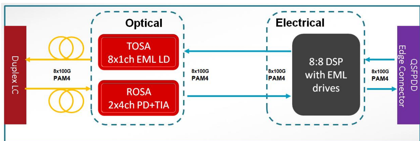
Figure1. Module Block Diagram
